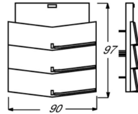
Control element Busch-triton® 6320/38
